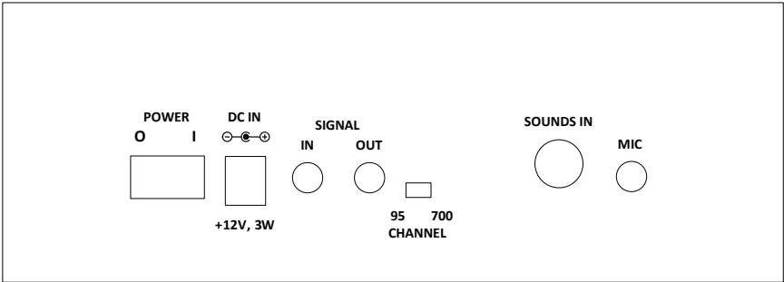
Figure 2: ISS Bottom Panel
