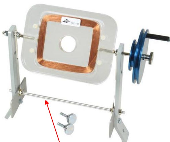
Fig. 1: Transport lock for the rotating induction coil
