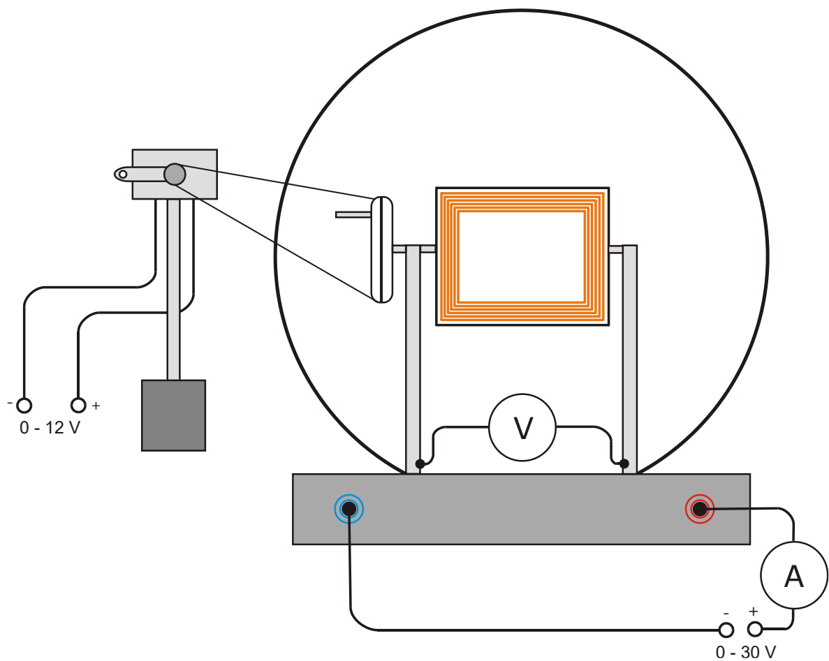
Fig. 2: Experiment set-up with rotating induction coil and driving motor
