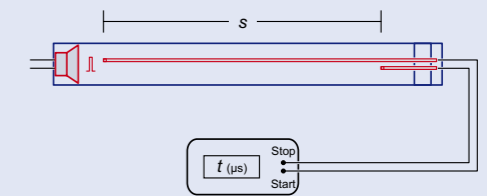
Fig. 1 Schematic of the experiment setup.
